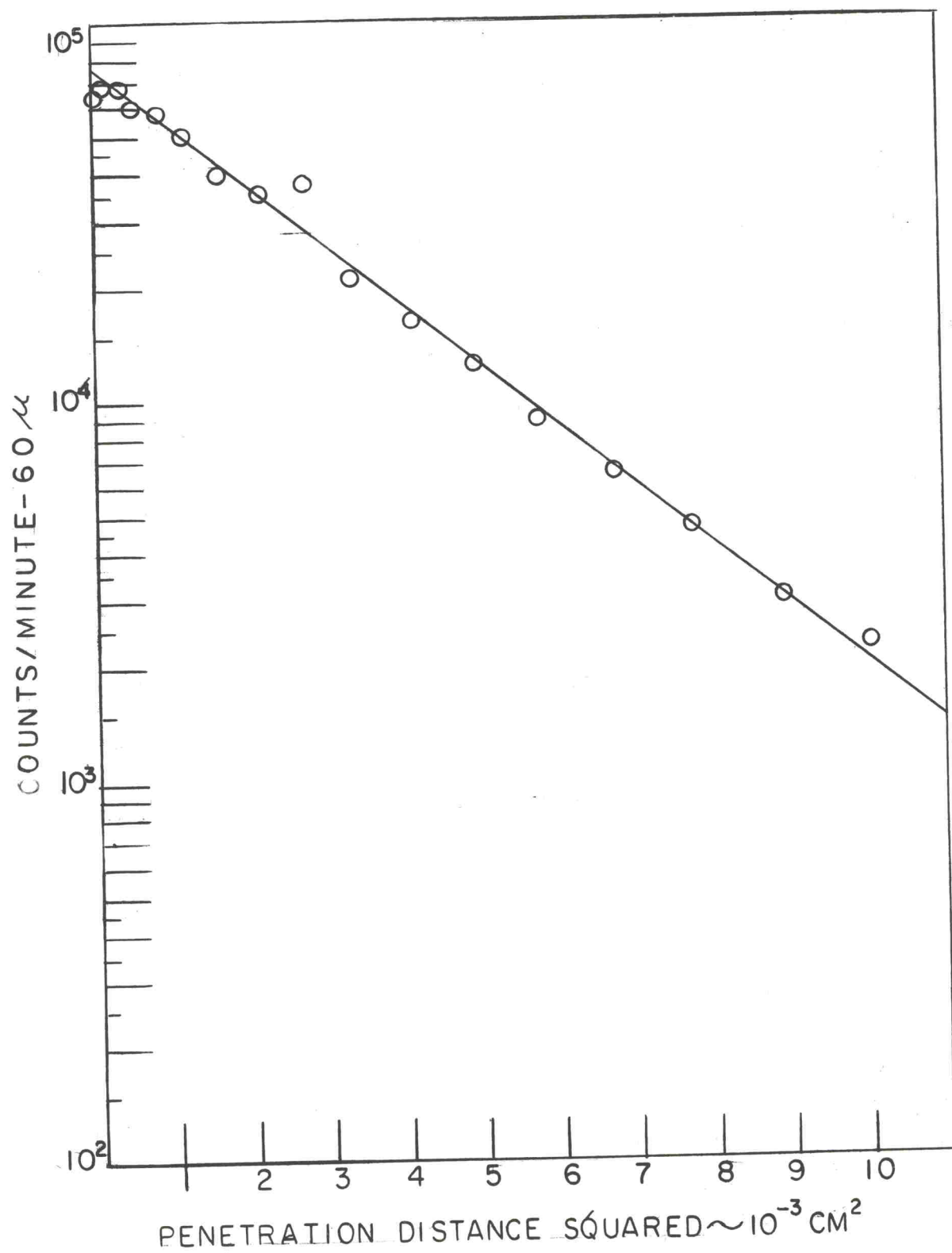
Figure 5. Solute Penetration Curve, Sample No. 68-- Annealed at 24 kb. pressure and 763°K for 3.18 \times 10^3 sec
